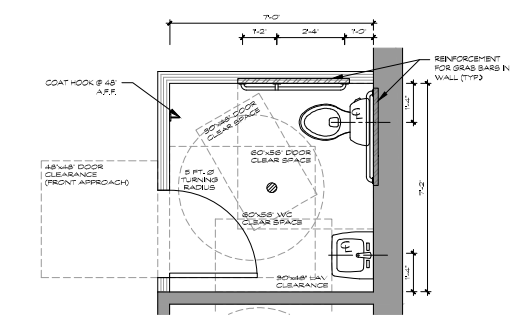
2 ACCESSIBLE TOILET PLAN 1/2" = 1'
