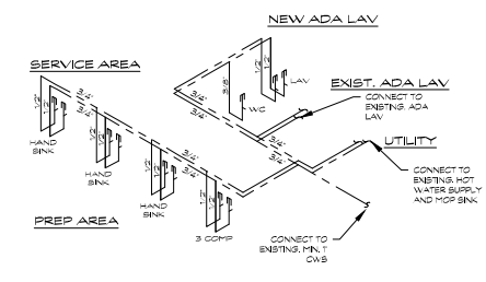
3 WATER SUPPLY DIAGRAM N.T.S.
